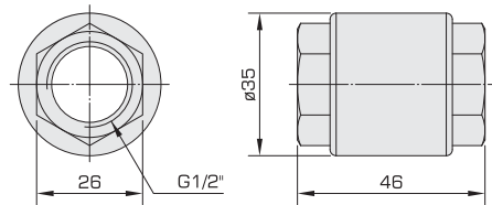
VC04 (G1/2")
